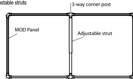
Top View System using 3-way corner post
